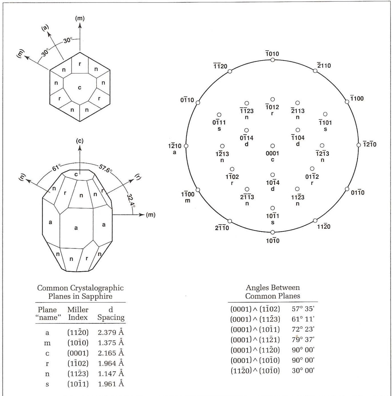
Figure 10. Representation of Sapphire ( \infty Al 2 O 3 ) Crystal Structures and Important Orientation Planes
